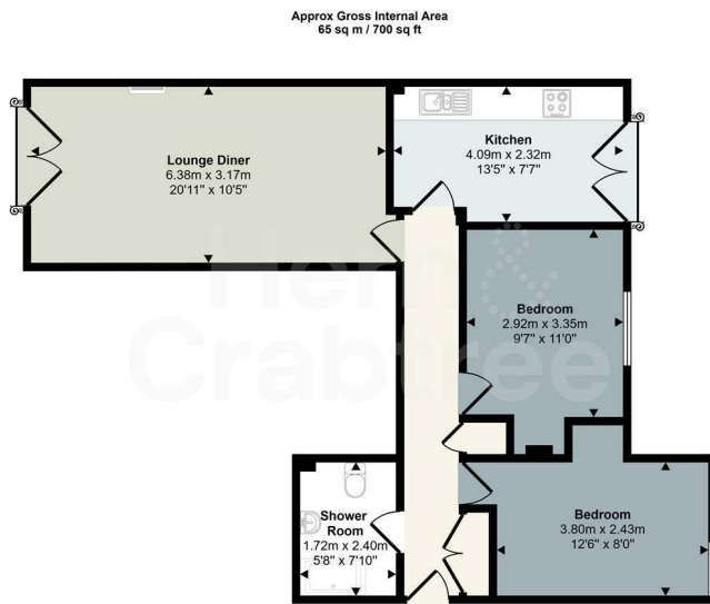
Floorplan
